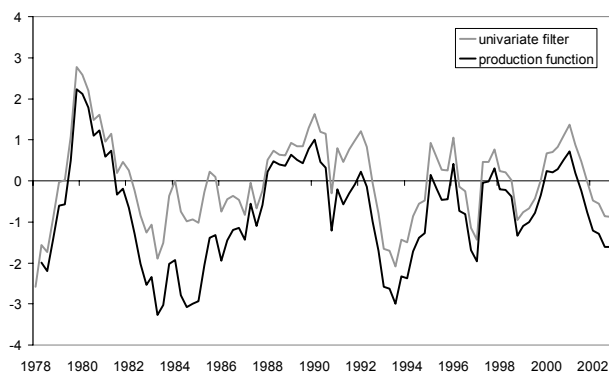
Graph 4 : Italy output gap estimates
