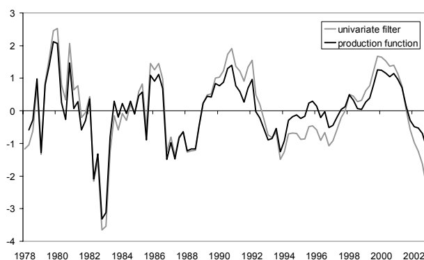
Graph 6 : Netherlands output gap estimates
