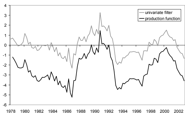
Graph 5 : Spain output gap estimates
