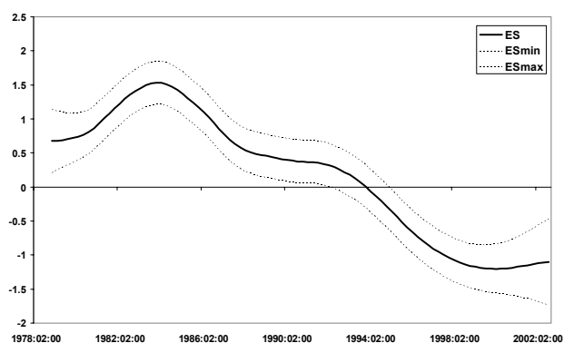
Graph 18 : Confidence band Spain
