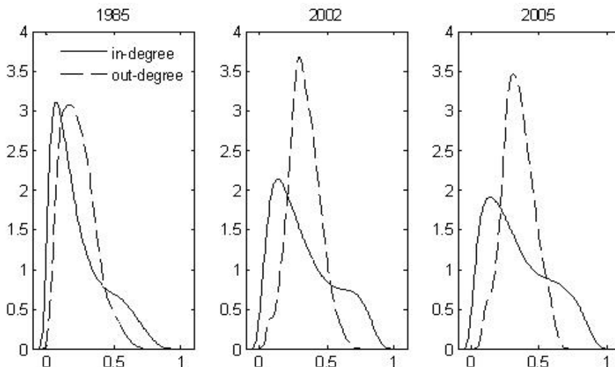
Figure 2: Degree distribution
