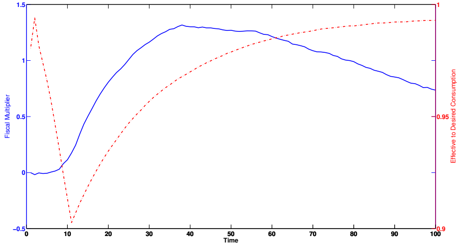
Figure 3: Evolution of fiscal multipliers (left scale) and ratio between actual and desired consumption (right scale). Deficit-spending rule.
