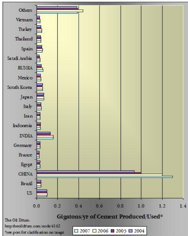
Figure 17 World cement production, 2004-2007
