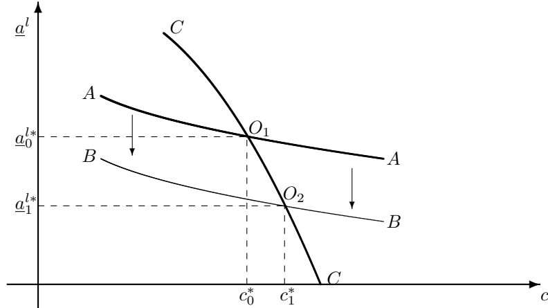
Figure 4: Steady state
