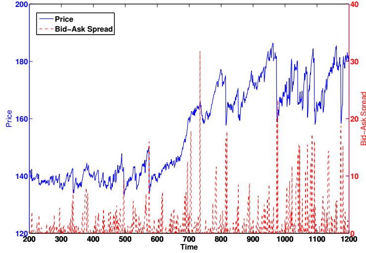
Figure 5: Evolution of asset price (solid line) and bid-ask spread (dashed line) in a single Monte-Carlo run.
