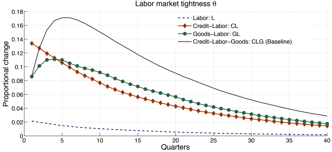
Figure 2: Comparing Frictions: Impulse Responses to a Positive Technology Shock across Models.
