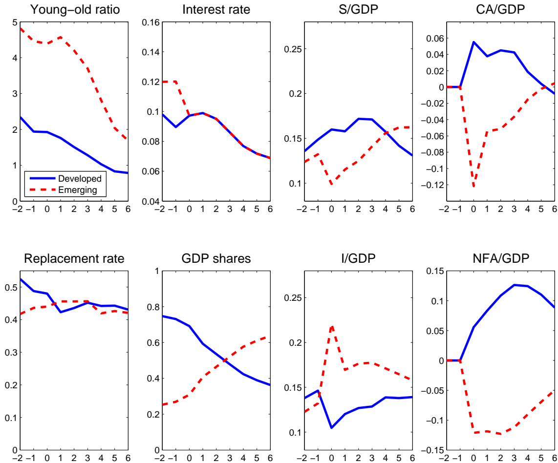
Figure 3.2: Capital Flows Between a Developed and an Emerging Region, Identical \tau and \theta Notes: The young-old ratio corresponds to the ratio of the size of the group of agents of age j = 1, 2 (i.e., 20-40) over the size of the group of agents of age j = 5, 6, 7 (i.e., 60-90). The values of calibrated parameters are given in Table 1.
