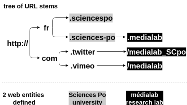
Figure 2: web entities are pointers to the URL name hierarchy.
