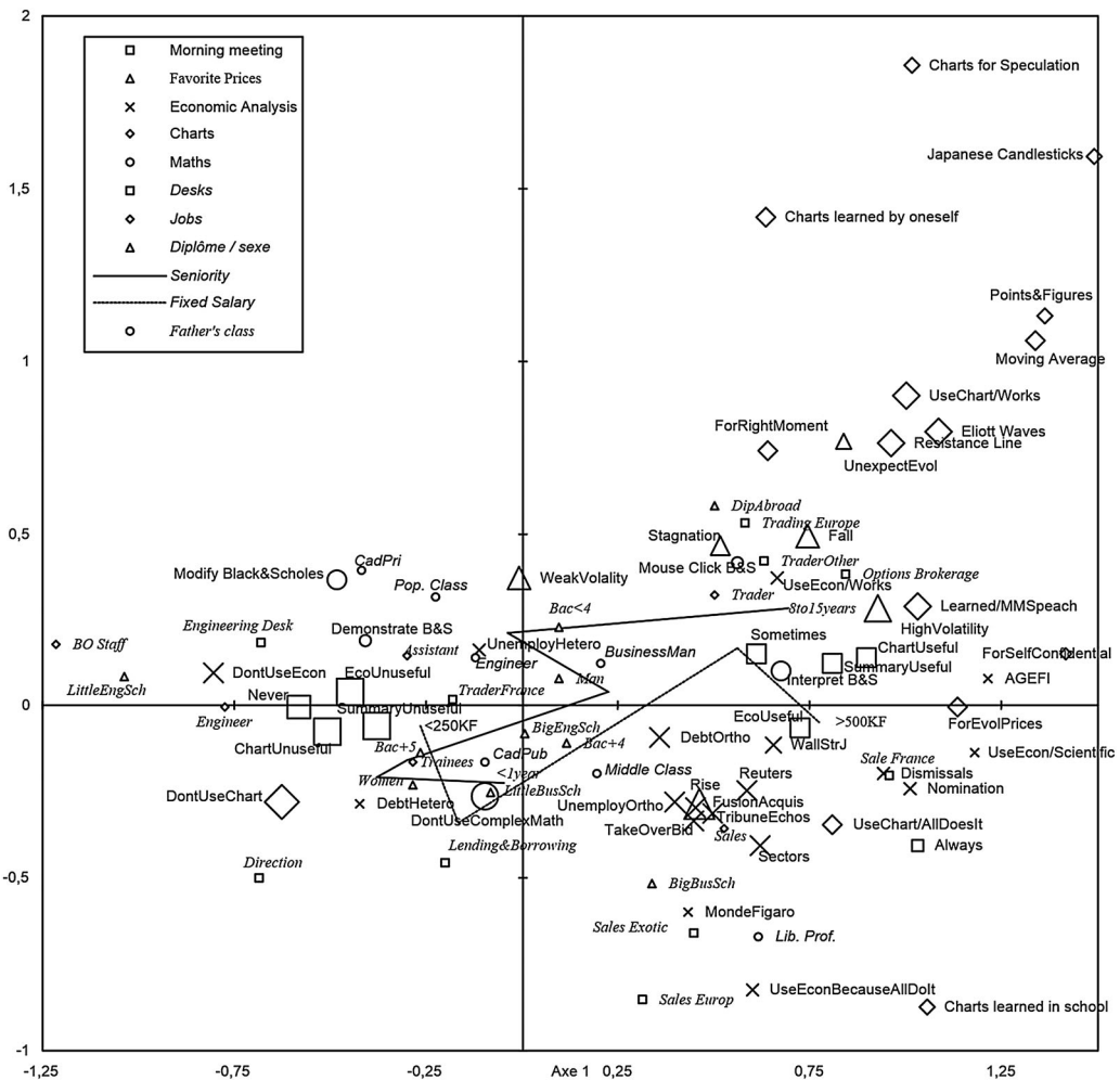
Figure 6. Multiple correspondence analysis of the winning strategies.
