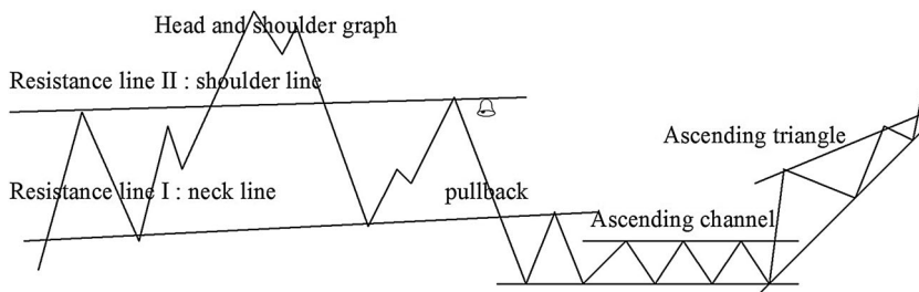
Figure 4. Prices with some basic chartist figures.
