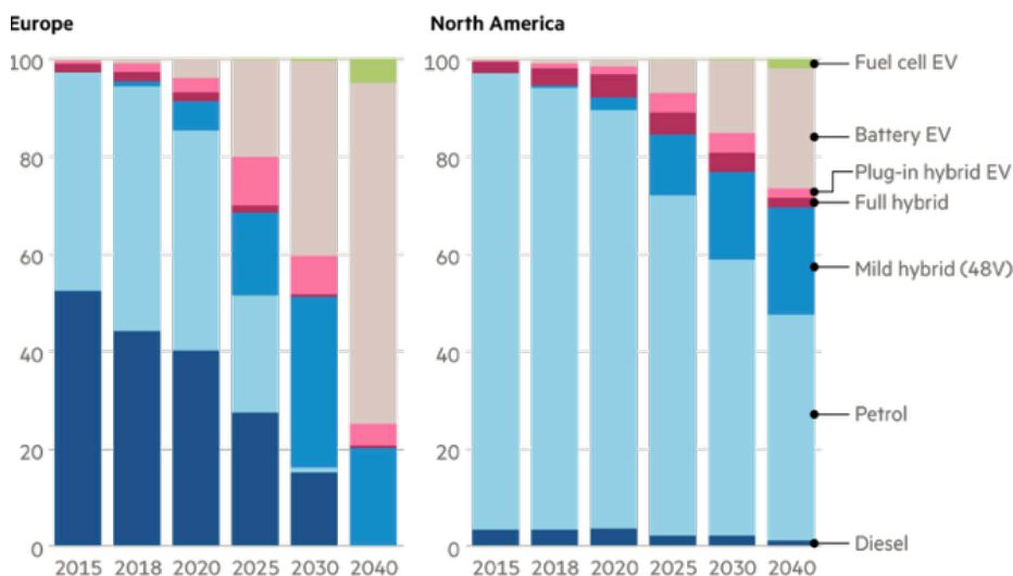
Powertrain split (%)
