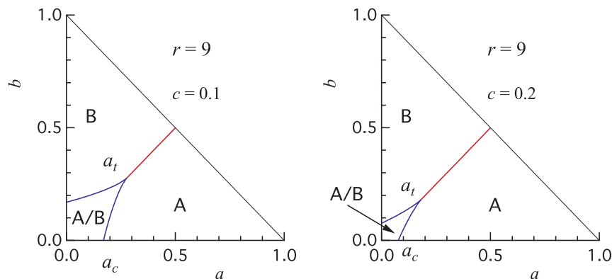
FIGURE 9 | Phase diagram on \{a, b\} plane for r = 9 . Left for c = 0.1 and right for c = 0.2 . The regions marked as A, B, and A/B represent parameter values with which the system converges unconditionally to A majority, unconditionally to B majority, and to either A or B majority depending on the initial configuration, respectively.
