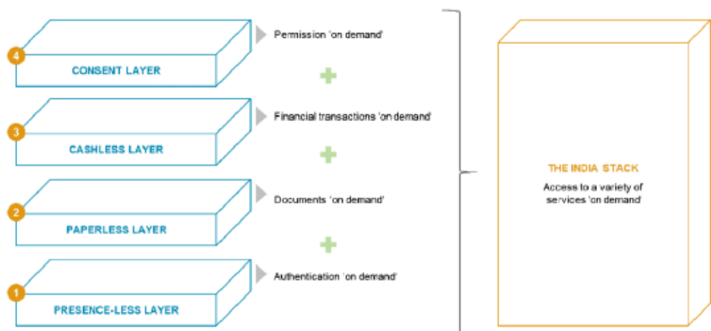
Figure 1: India Stack
