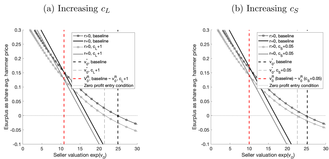
Figure H.2. : Numerical simulations: minimal effect endogenizing v_0^R
