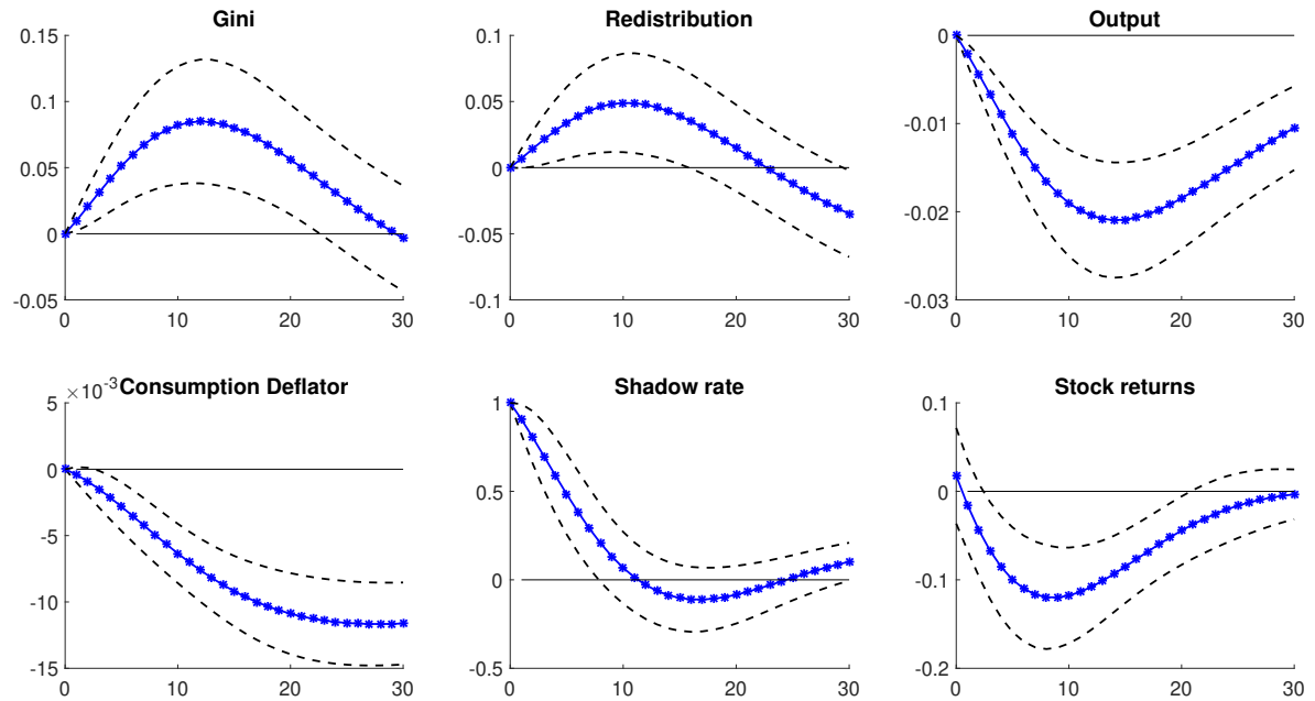
Figure 30: Responses to a shock on the shadow rate, VAR(6)
