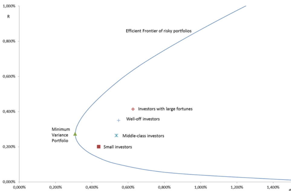
Figure 2. Advised portfolios and the efficient frontier.
