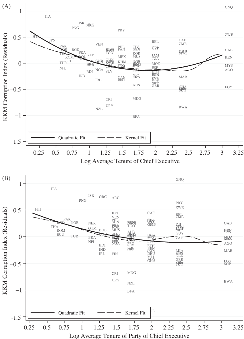
Figure 2. The U-shape between corruption and average incumbent tenure (cross-section). (A) Log executive tenure. (B) Log party tenure.
