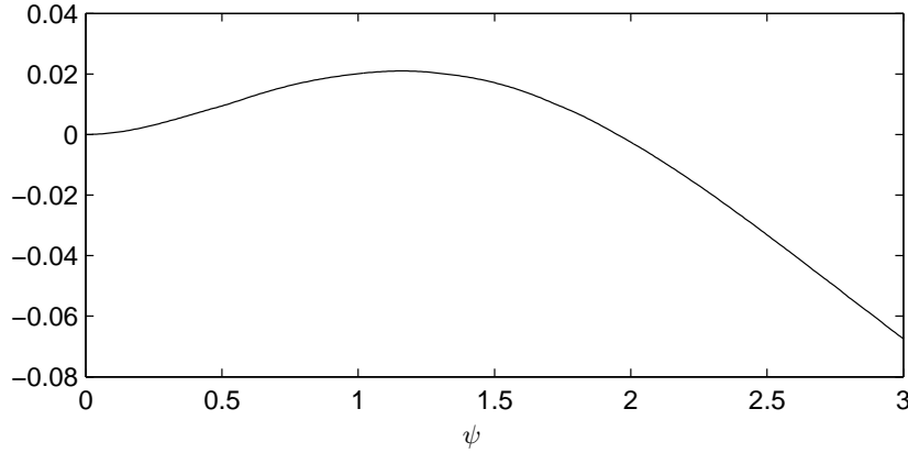
Asymptotic bias of \hat{\psi}_a when \lambda_i \sim N(0, 1) .
