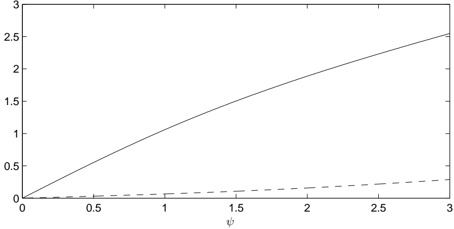
Figure 1. Asymptotic biases in the probit model, m = 2
