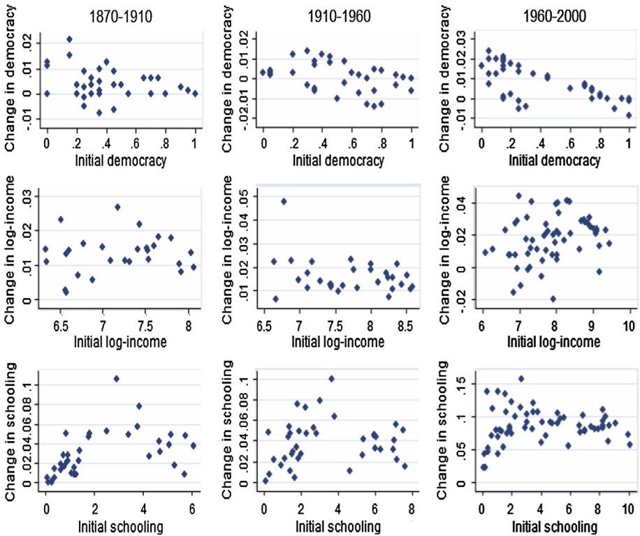
Fig. 4 Convergence in democracy, GDP per capita and average years of schooling by period
