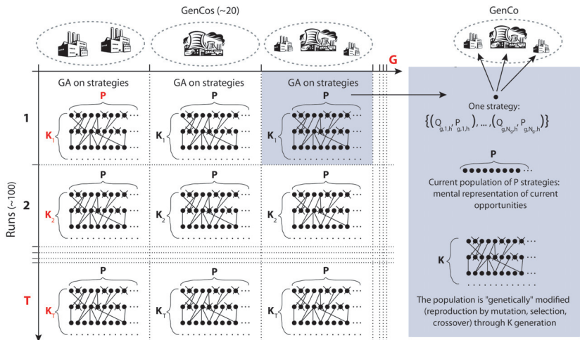
Figure 2. A schematic representation of the learning algorithm
