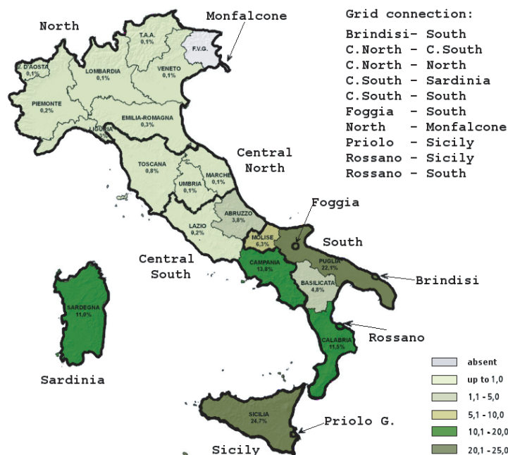
Figure 1. Map of Italy showing the regional distribution of installed wind capacity (in varying degrees of green) and the borders between zones in the transmission grid (thick black lines)*
