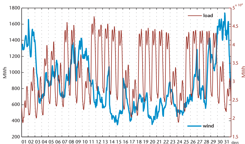
Figure 3. Time series of electricity demand and wind supply, Italy, January 2010
