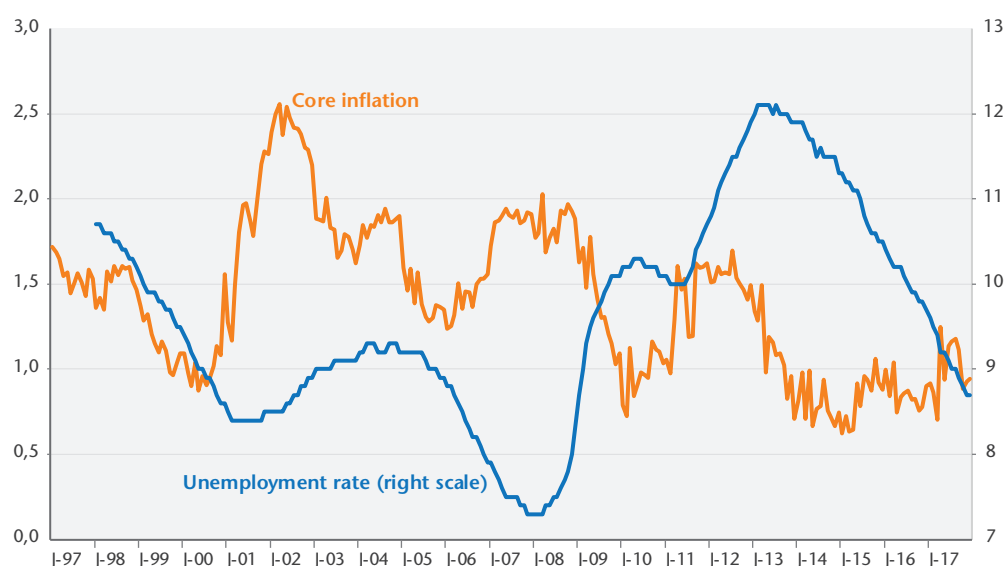
Figure 4. Core inflation and unemployment rate in the euro area
