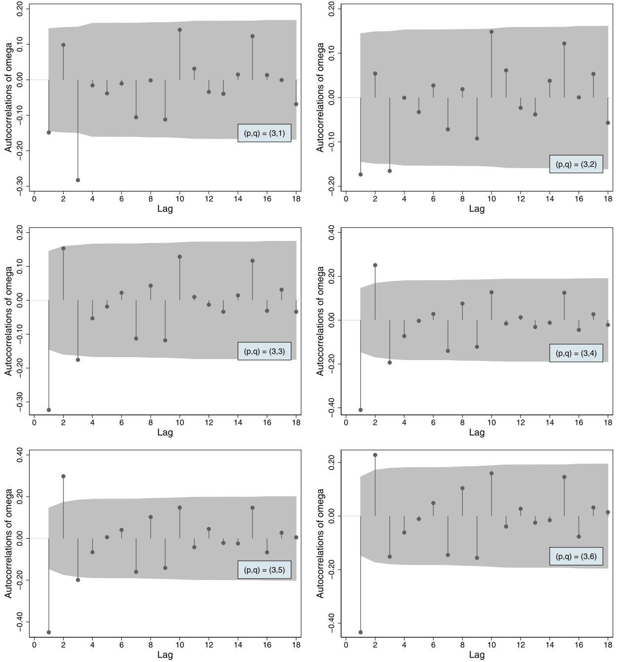
Fig. 2. Autocorrelograms of estimated residuals from (7).
