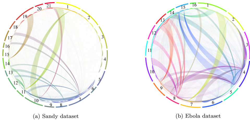
Figure 2: Collaboration networks
