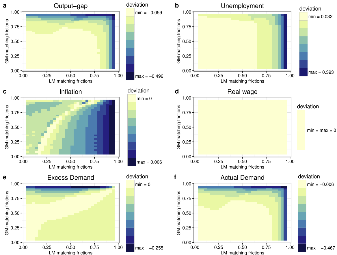
Fig. 7. Fixed real-wages simulation. Effects of a variation in the quality of matching in the labor (horizontal dimension) and in the goods markets (vertical dimension). From left/bottom to right/top the quality of matching deteriorates.
