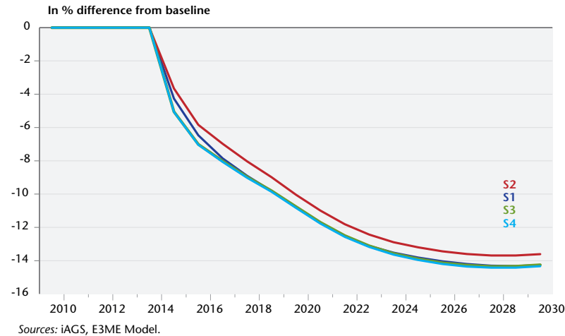
Figure 9. EU28 CO2 emissions by scenario,
