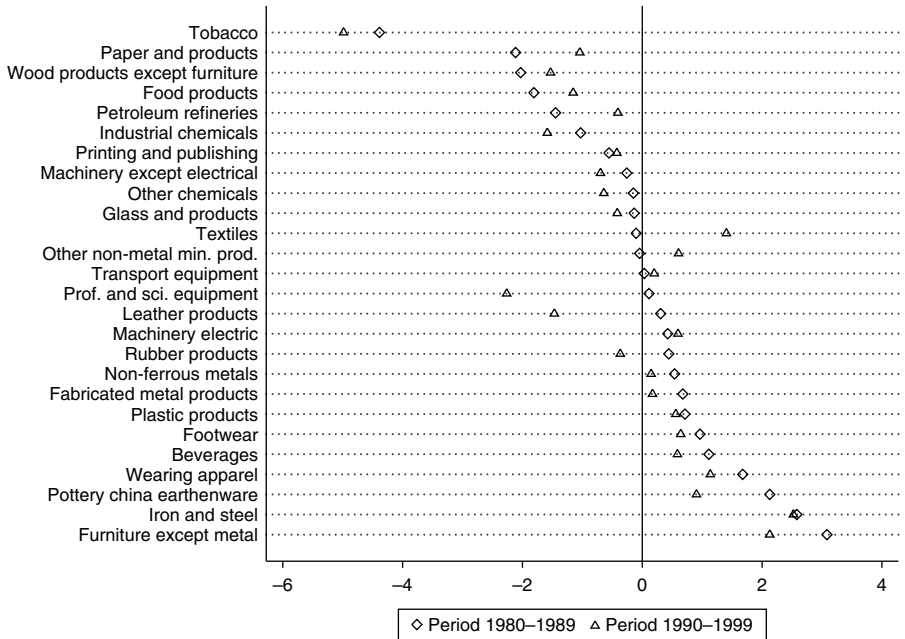
FIGURE 7 Asymmetries in border coefficients: (US \rightarrow EU9)-(EU9 \rightarrow US)
