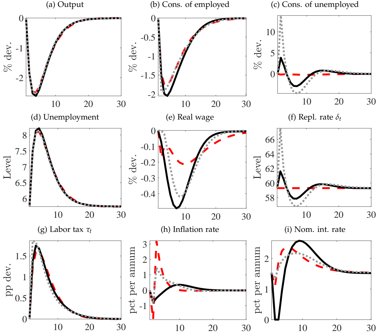
Figure 4: Optimal responses to a large positive separation shock.
