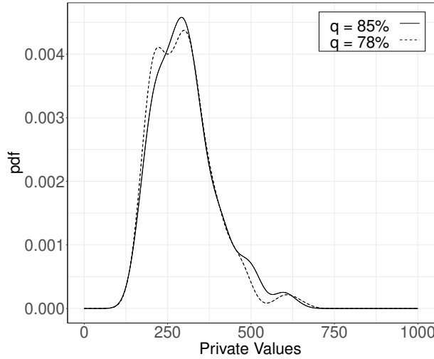
Figure 3: Out-of-sample validation
