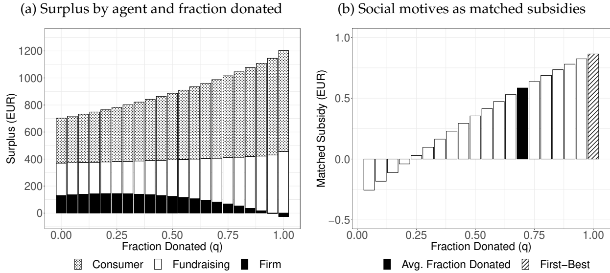
Figure 7: Welfare analysis
