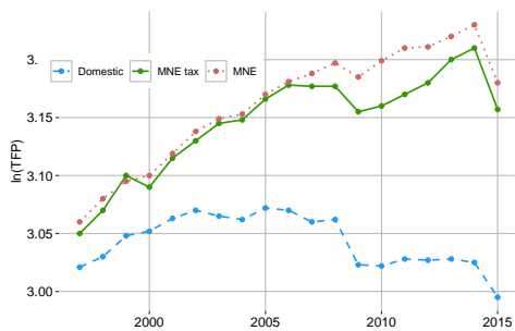
Figure 5: TFP levels
