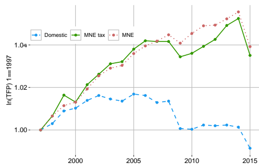
Figure 6: TFP evolution
