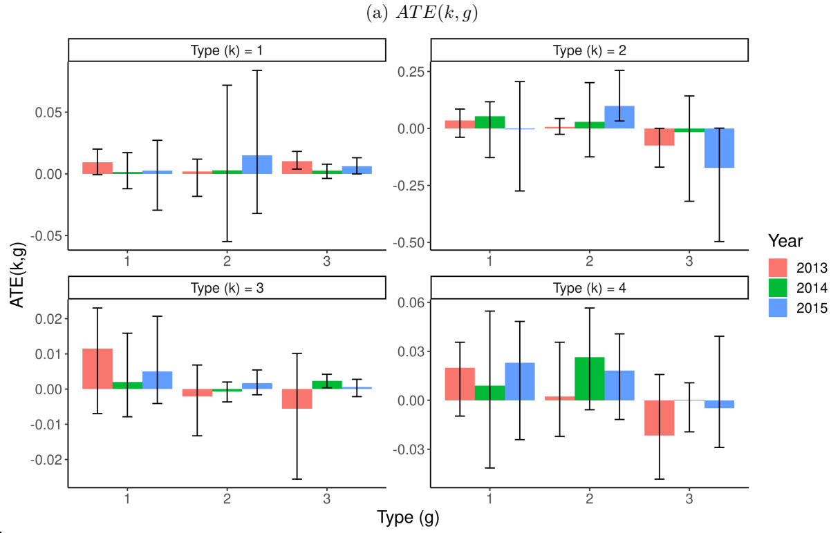
Figure 7: Type-conditional treatment effects
