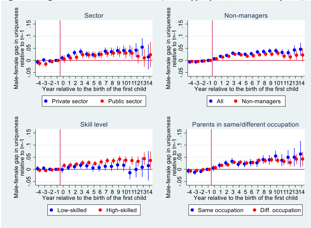
Figure A7 Figure 2 with alternative cutoffs ( \leq 3 in upper panel, \leq 7 in lower panel)
