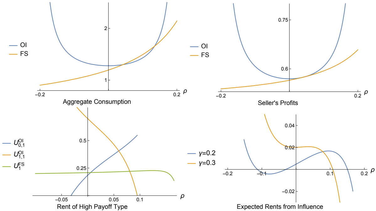
Figure 6: Observable influence in the 2x2 consumption example.
