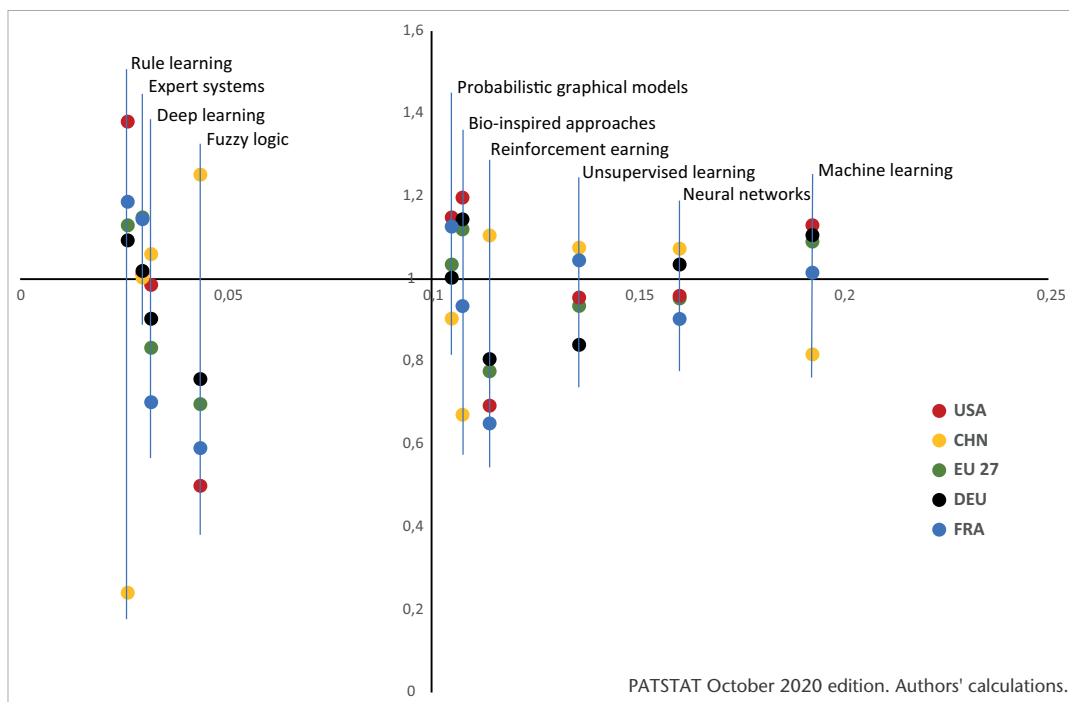
Figure 3. Strategic positioning of countries by AI technique
