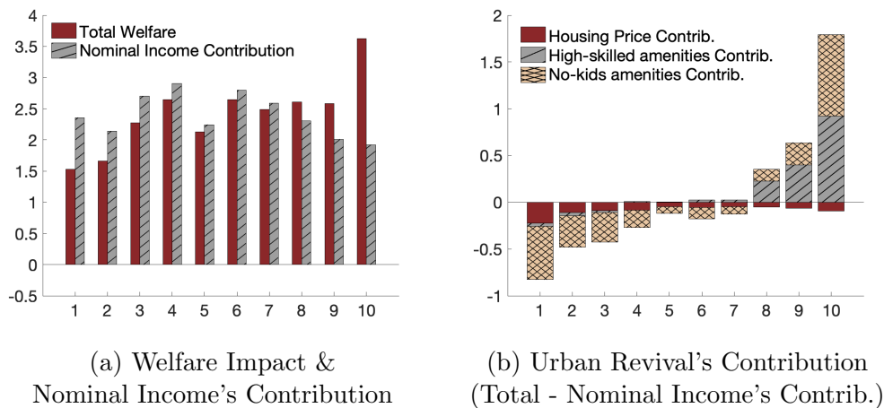
Figure 13: Decomposing the Welfare Impact of the Delay Premium
