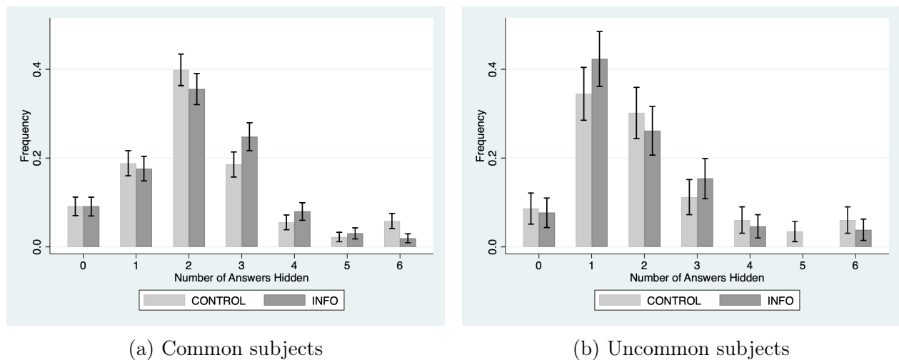
Figure 4: Hiding 0 to 6 answers, per treatment for the MAR target
