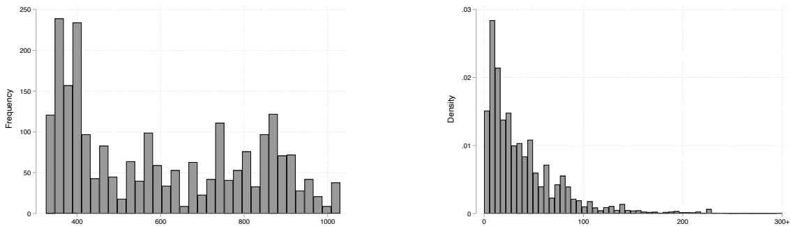
(a) Distribution of hoards by tpq , AD 325-950
