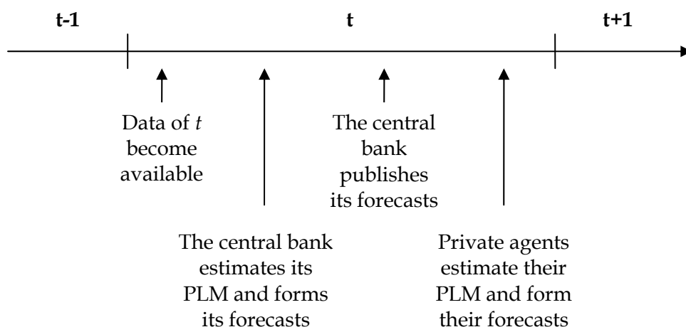
Figure A: the timing of decisions
