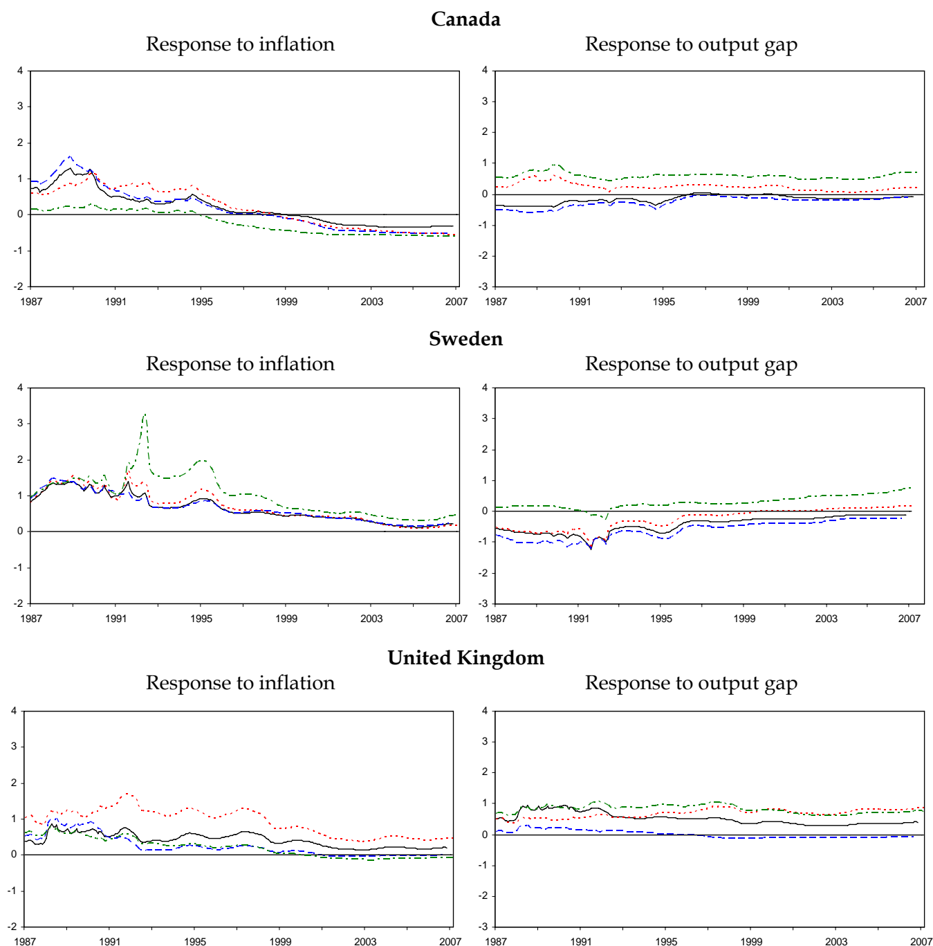
Figure IV.4 – Time-Varying Responses to Inflation and Output Gap with an Alternative Noise-to-Variance ratio = 0.001
