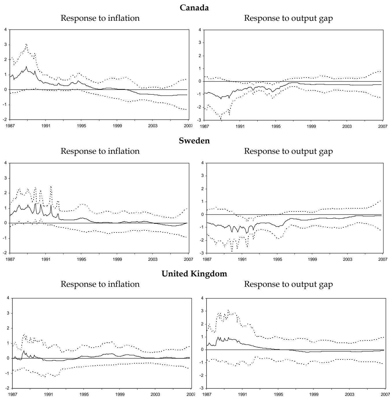
Figure IV.2 – Time-Varying Responses to Inflation and Output Gap with h_{\pi} = h_y = 9 , a Noise-to-Variance ratio = 0.01 and 1 S.E. bands
